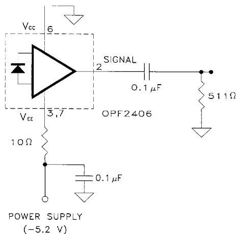
Recommended AC Coupled Receiver Circuit
