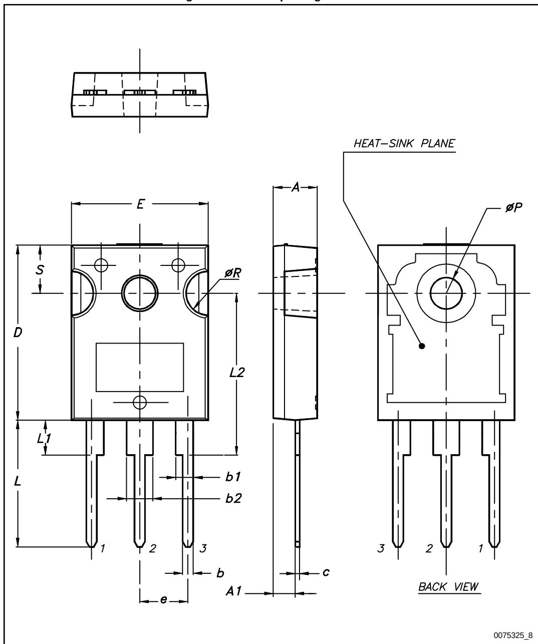
Figure 29: TO-247 package outline
