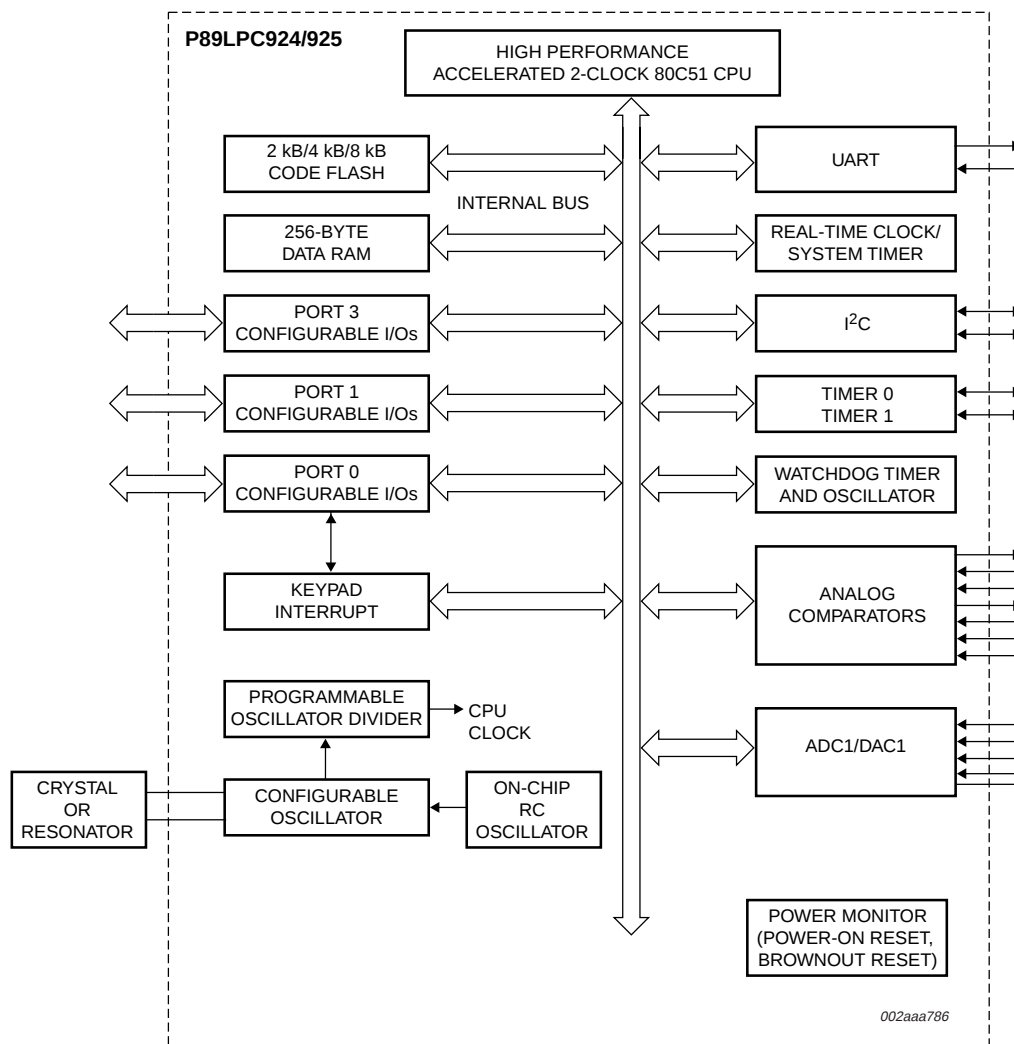
Fig 1. Block diagram.
