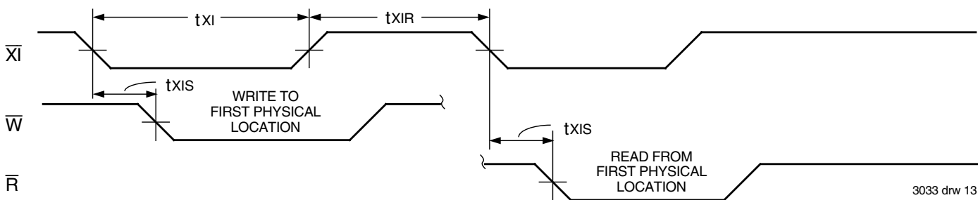
Figure 11. Expansion In
