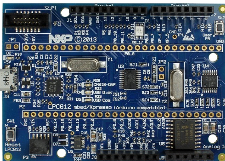
Figure 1.4. LPC800-MAX Board
