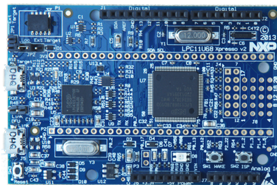
Figure 1.3. LPCXpresso V2 Board (LPCXpresso11U68)
