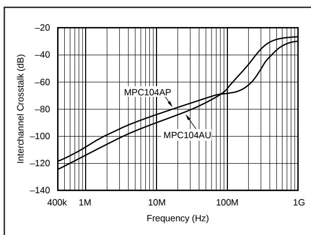
FIGURE 5. Interchannel Crosstalk.
