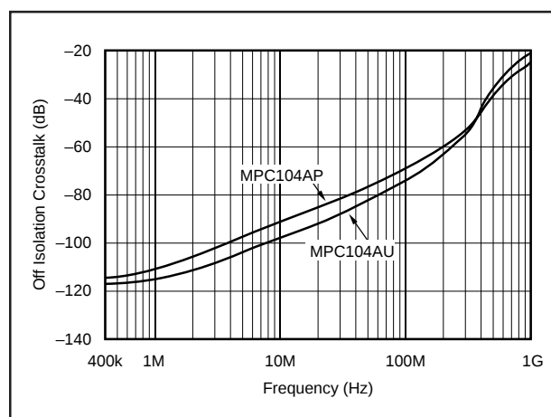
FIGURE 6. Off Isolation.
