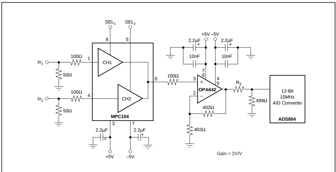
FIGURE 11. High-Speed Data Acquisition System.
