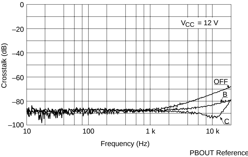
Crosstalk vs. Frequency (PB MODE R→L)
