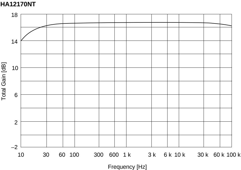
Total Gain vs. Frequency (REC MODE RECOUT NR-OFF V_{CC} = 14 V)
