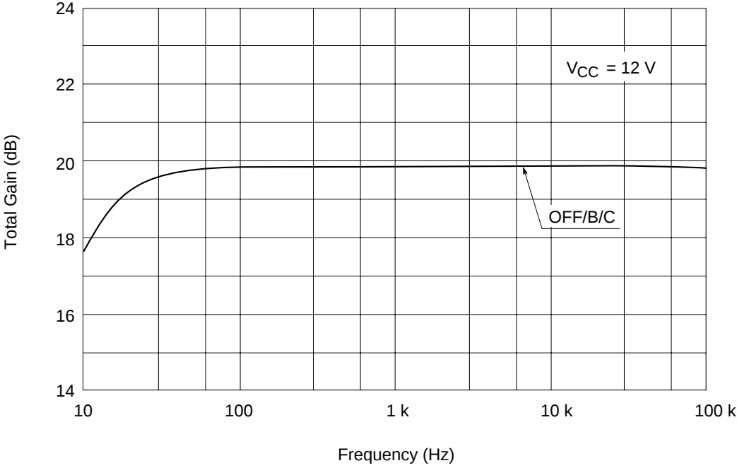
Total Gain vs. Frequency (PB MODE RECOU)
