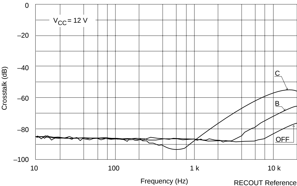
Crosstalk vs. Frequency (REC MODE R \leftrightarrow L)
