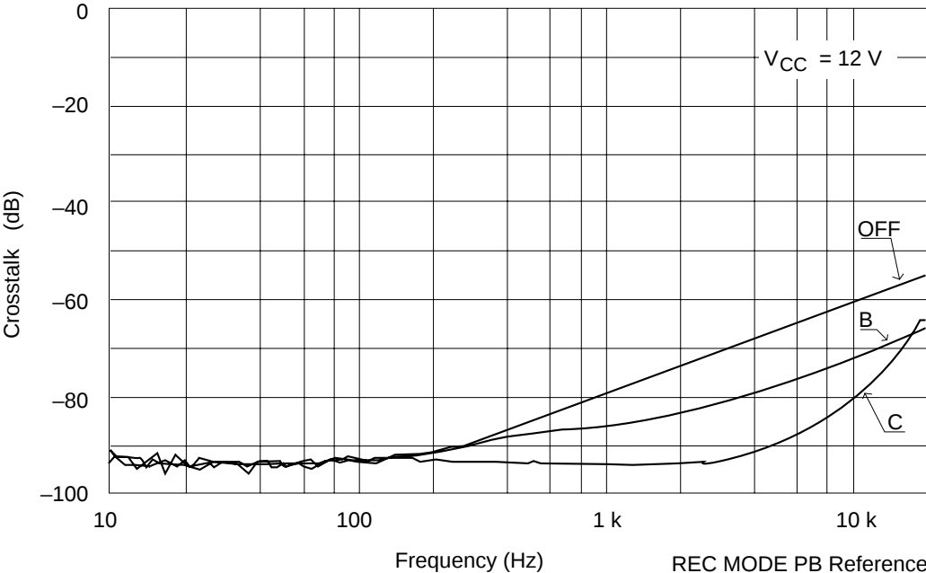
Crosstalk vs. Frequency (REC MODE PB→PB)
