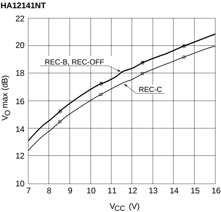
Maximum Output Level vs. Supply Voltage (REC MODE)
