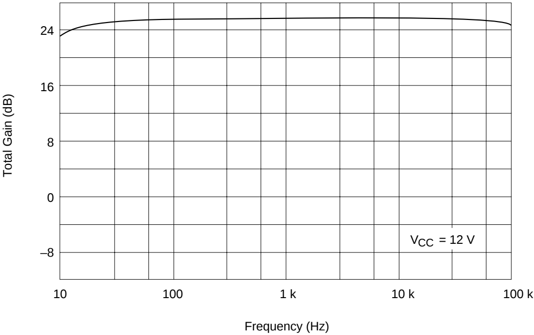
Total Gain vs. Frequency (PB MODE PBOU NR-OFF)
