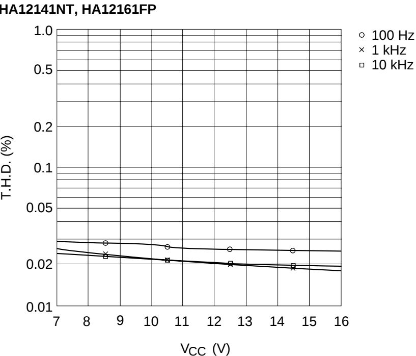
Total Harmonic Distortion vs. Supply Voltage (PB MODE NR-B)
