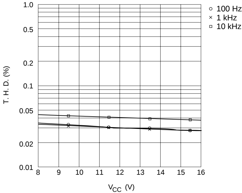
HA12142NT, HA12162FP
