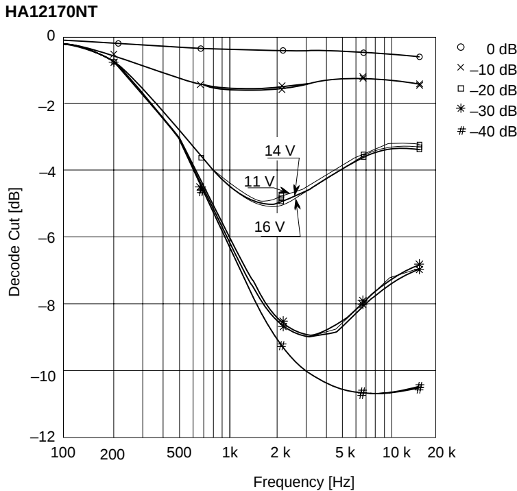
Decode Cut vs. Frequency (NR-B V_{CC} = 11 V, 14 V, 16 V)
