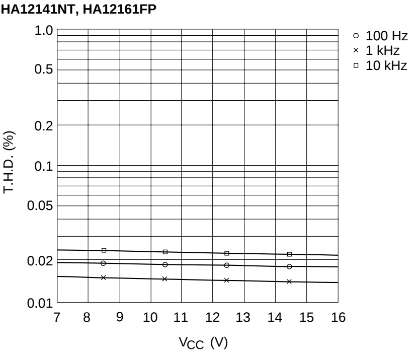
Total Harmonic Distortion vs. Supply Voltage (PB MODE NR-OFF)
