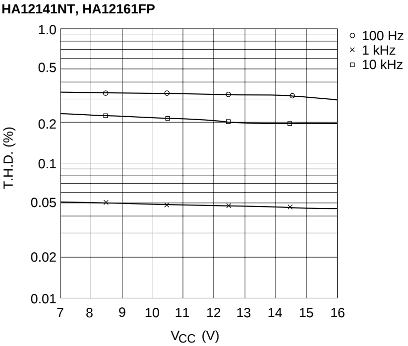
Total Harmonic Distortion vs. Supply Voltage (PB MODE NR-C)
