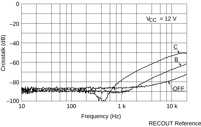
Crosstalk vs. Frequency (REC MODE R→L)
