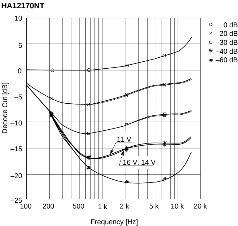
Decode Cut vs. Frequency (NR-C V_{CC} = 11 V, 14 V, 16 V)
