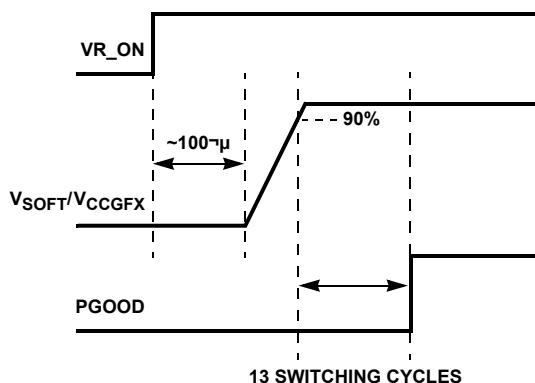
FIGURE 4. ISL6263A START-UP TIMING
