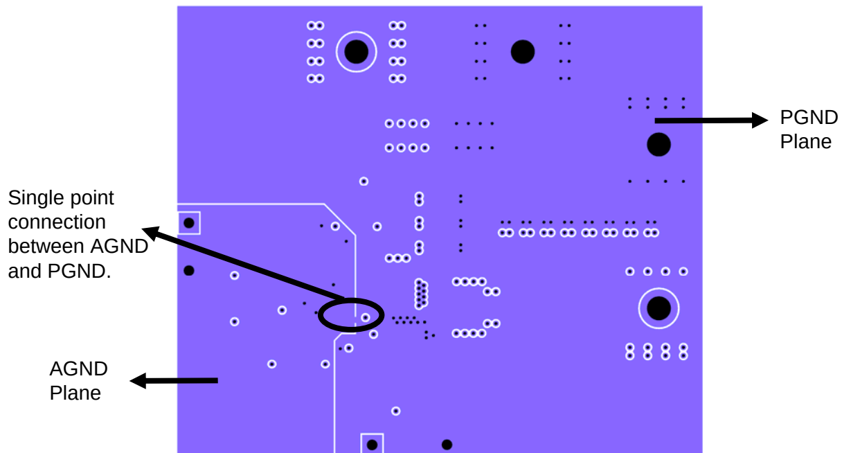
Fig. 4: Board layout, mid-layer I.
