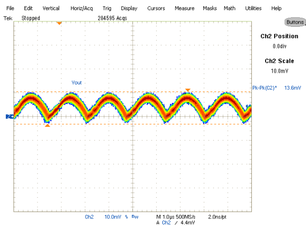
Fig. 10: Output Voltage Ripple, 8A load Ch 2 :V out
