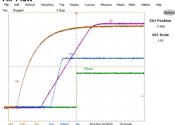
Fig. 8: Start up at 8A Load, Ch 1 :V in , Ch 2 :V out , Ch 3 :V ss , Ch 4 :V PGGood
