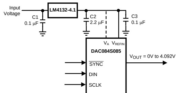
Figure 38. LM4130 as a Power Supply
