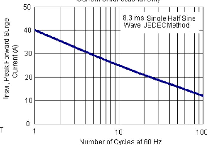
Fig. 4 Maximum Non-Repetitive Forward Surge Current Unidirectional Only
