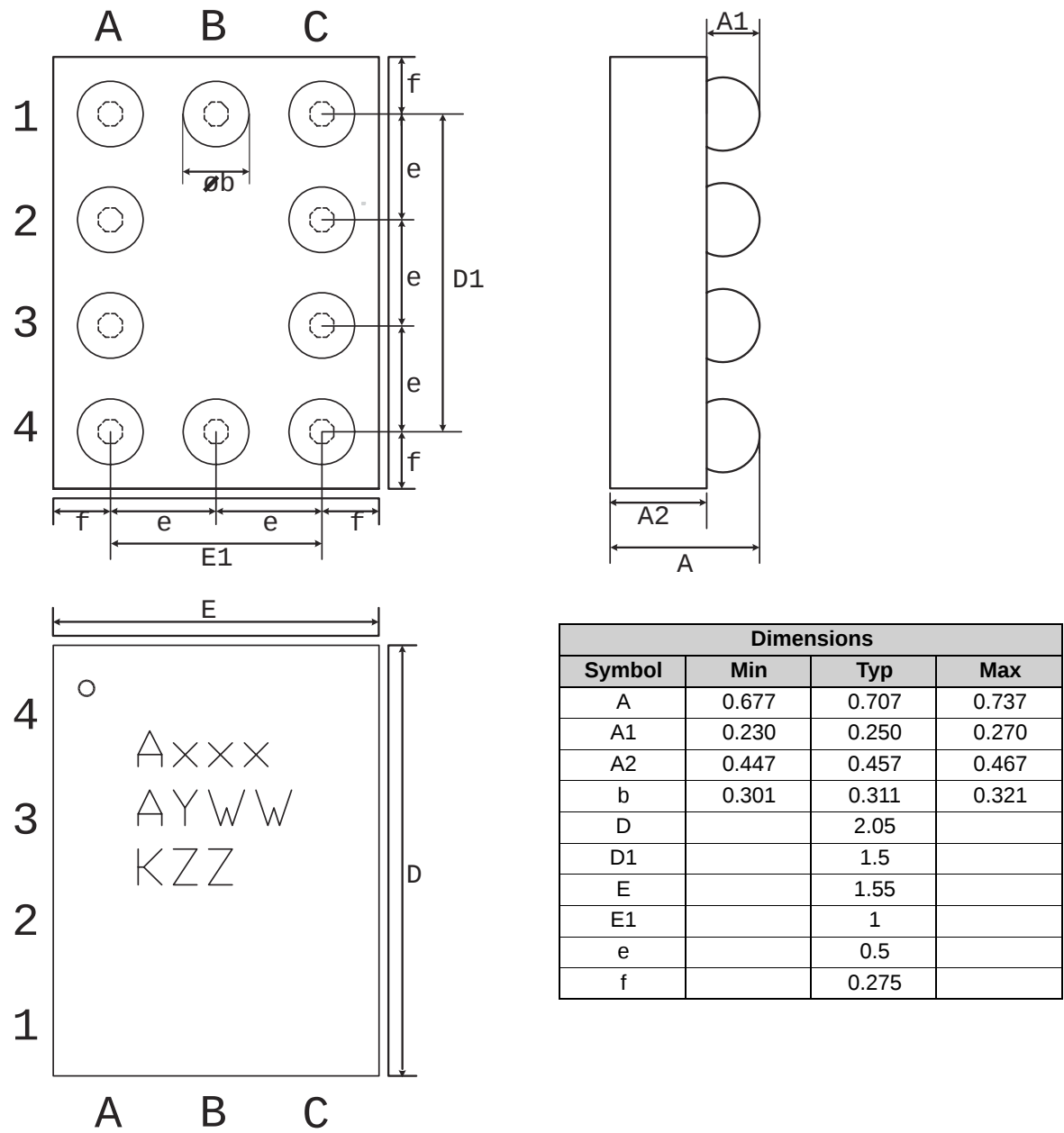
Figure 23. WL-CSP-10 Package
