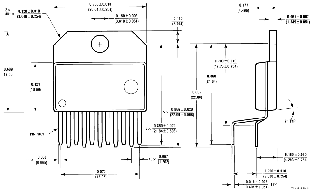
NS Package Number TA11B Order Number LM2415T
