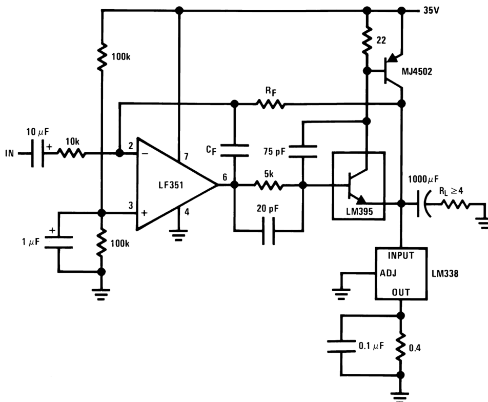
Figure 7-26. Power Amplifier
