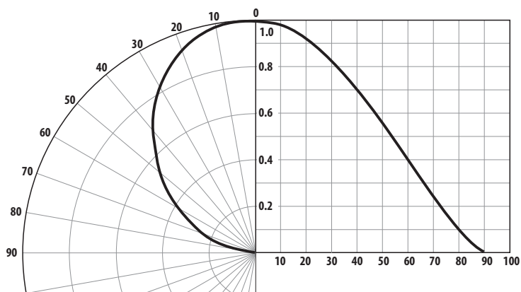
Figure 6. Relative luminous intensity vs. angular displacement.
