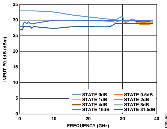
Figure 28. Input P0.1dB vs. Frequency (Major States Only)
