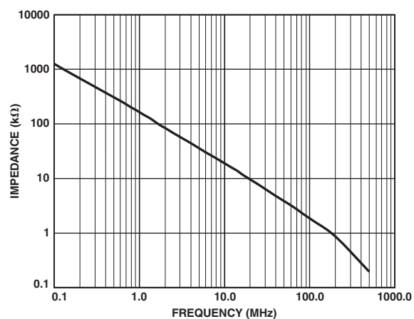
TPC 22. AD8187 Input Impedance vs. Frequency
