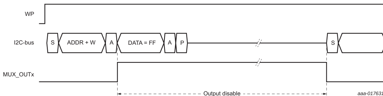
Fig 8. Write when WP disabled
