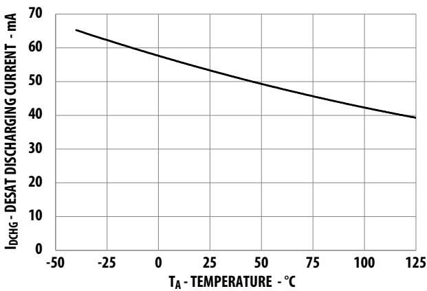
Figure 11 I_{DSCHG} across Temperature
