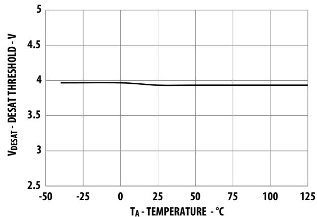
Figure 10 V_{DESAT} Threshold across Temperature
