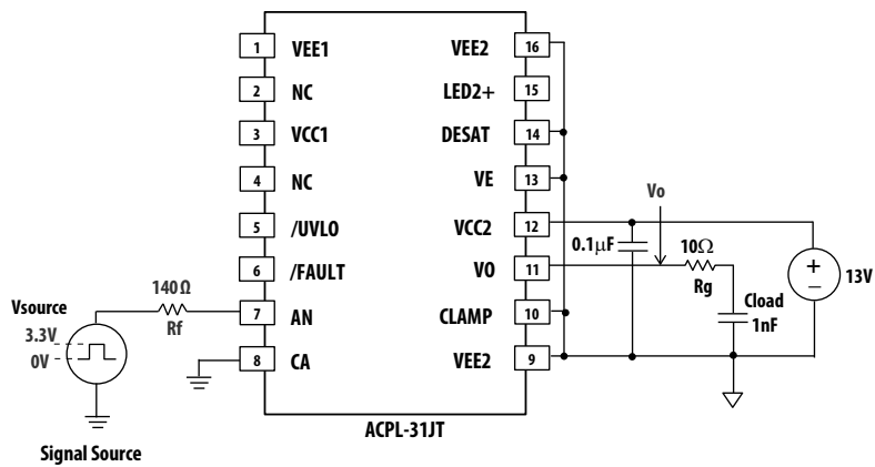
Figure 12 Propagation Delay Test Circuit and Timing Diagram
