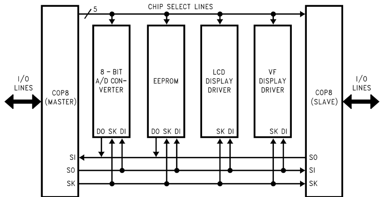
Figure 36. MICROWIRE/PLUS Application
