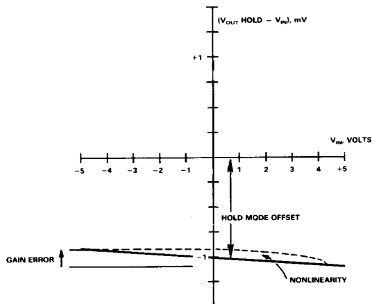
Figure 3. Hold Mode Offset, Gain Error and Nonlinearity
