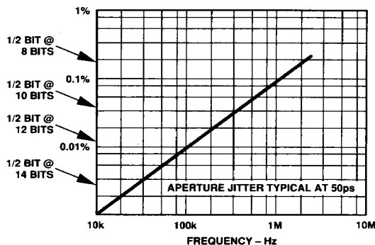
Figure 6. Error Magnitude vs. Frequency
