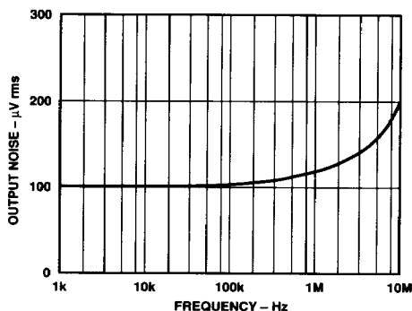
Figure 5. RMS Noise vs. Input Bandwidth of ADC
