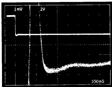
Figure 2. Typical AD781 Hold Mode
