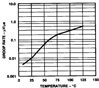
Droop Rate vs. Temperature, V_{IN} = 0 V
