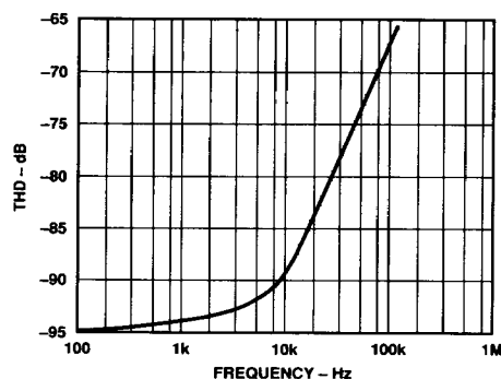
Figure 7. Total Harmonic Distortion vs. Frequency
