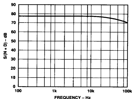
Figure 8. Signal/(Noise and Distortion) vs. Frequency
