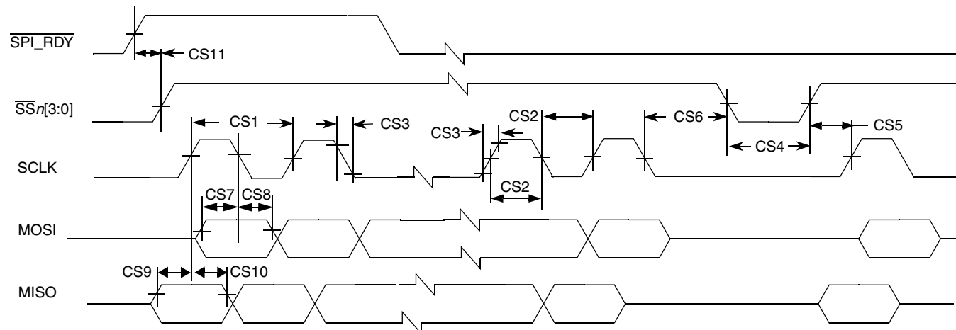
Figure 7. CSPI Master Mode Timing Diagram
