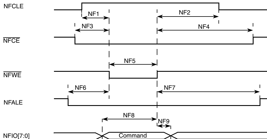
Figure 11. Command Latch Cycle Timing Diagram
