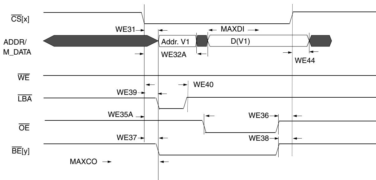
Figure 23. Asynchronous A/D muxed Read Access (RWSC = 5)
