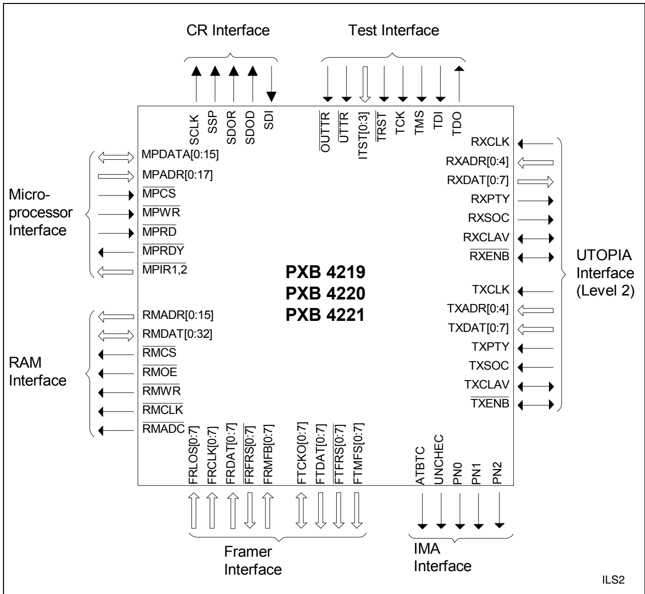
Figure 1 Logic Symbol
