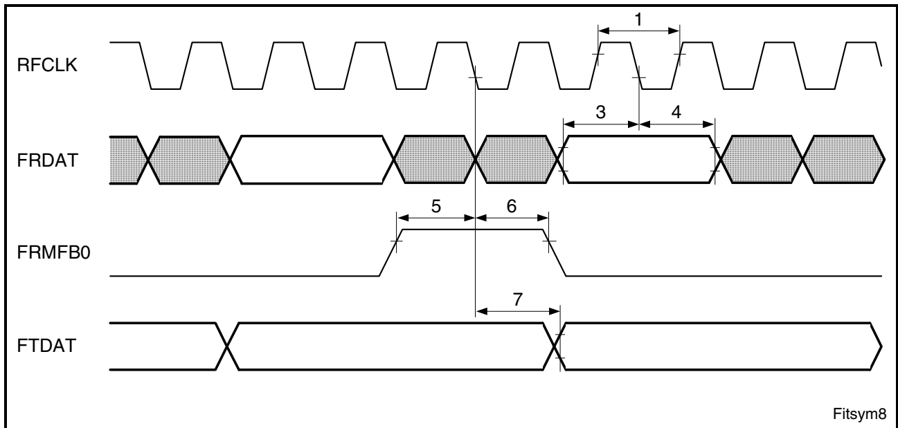
Figure 62 Framer Interface Timing in SYM 8.192 MHz
