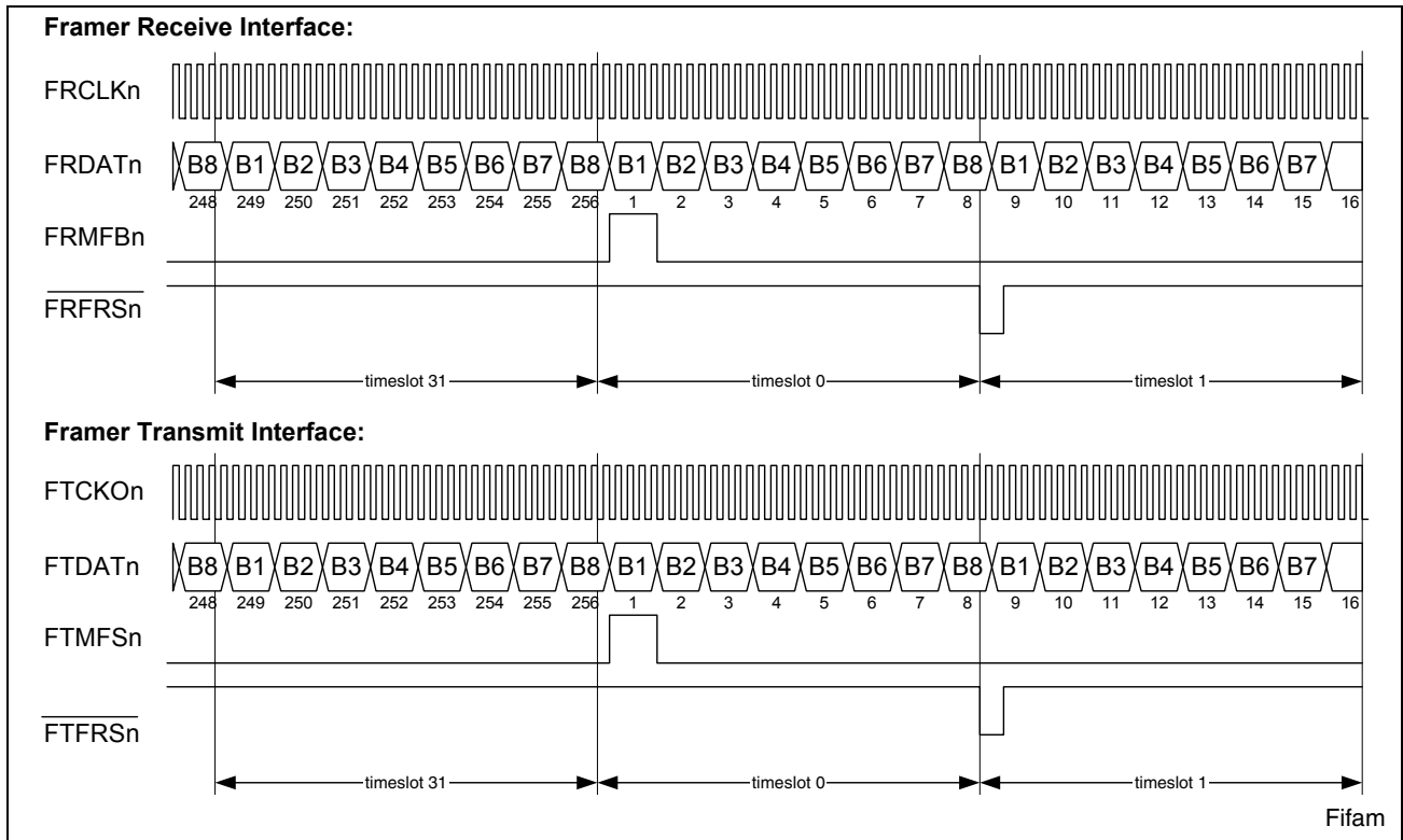
Figure 23 Framers Interface in FAM
