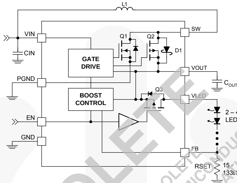
Figure 2. Block Diagram
