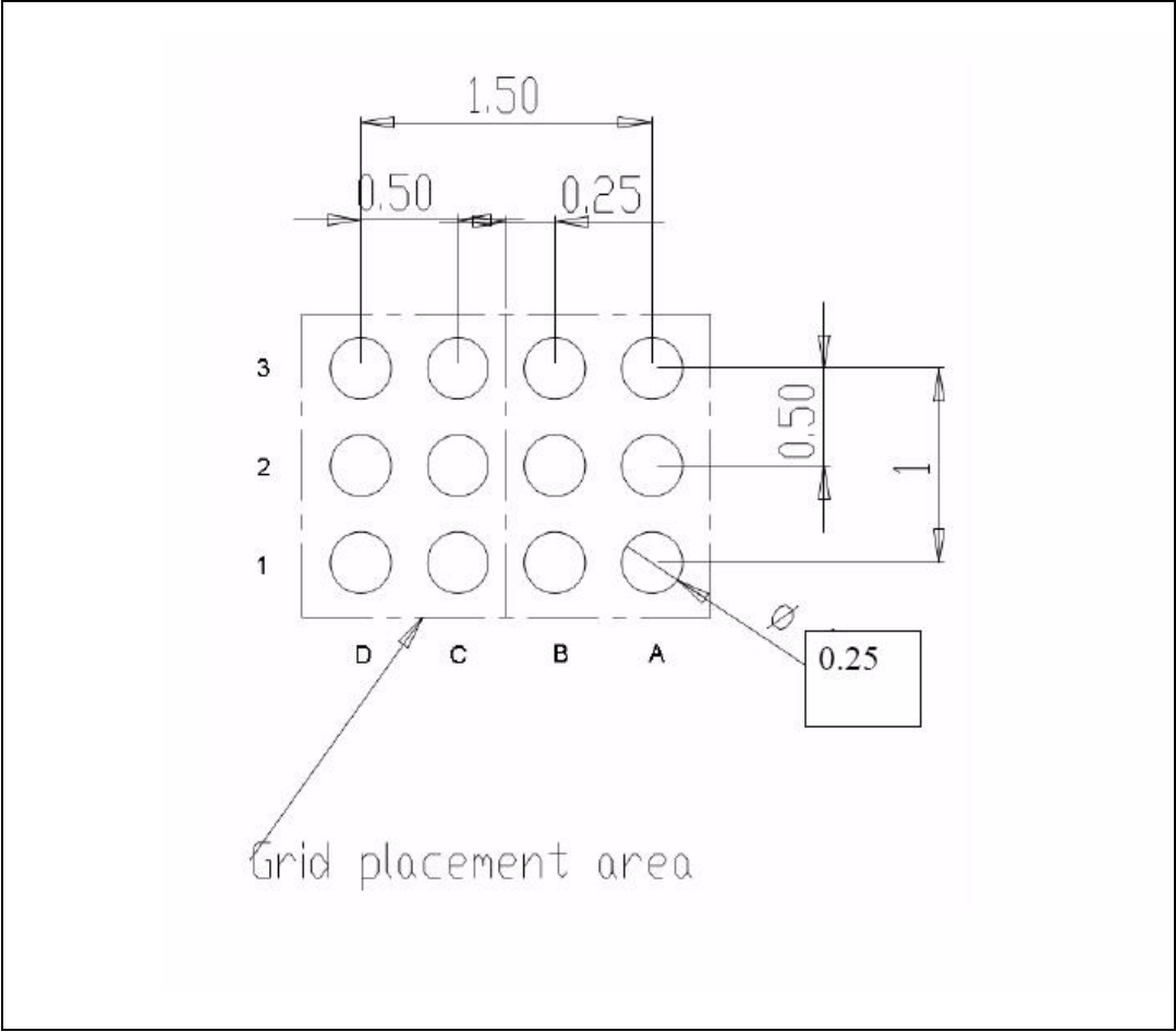
Figure 10. Footprint recommendation
