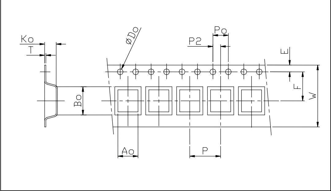
Figure 11. Tape information
