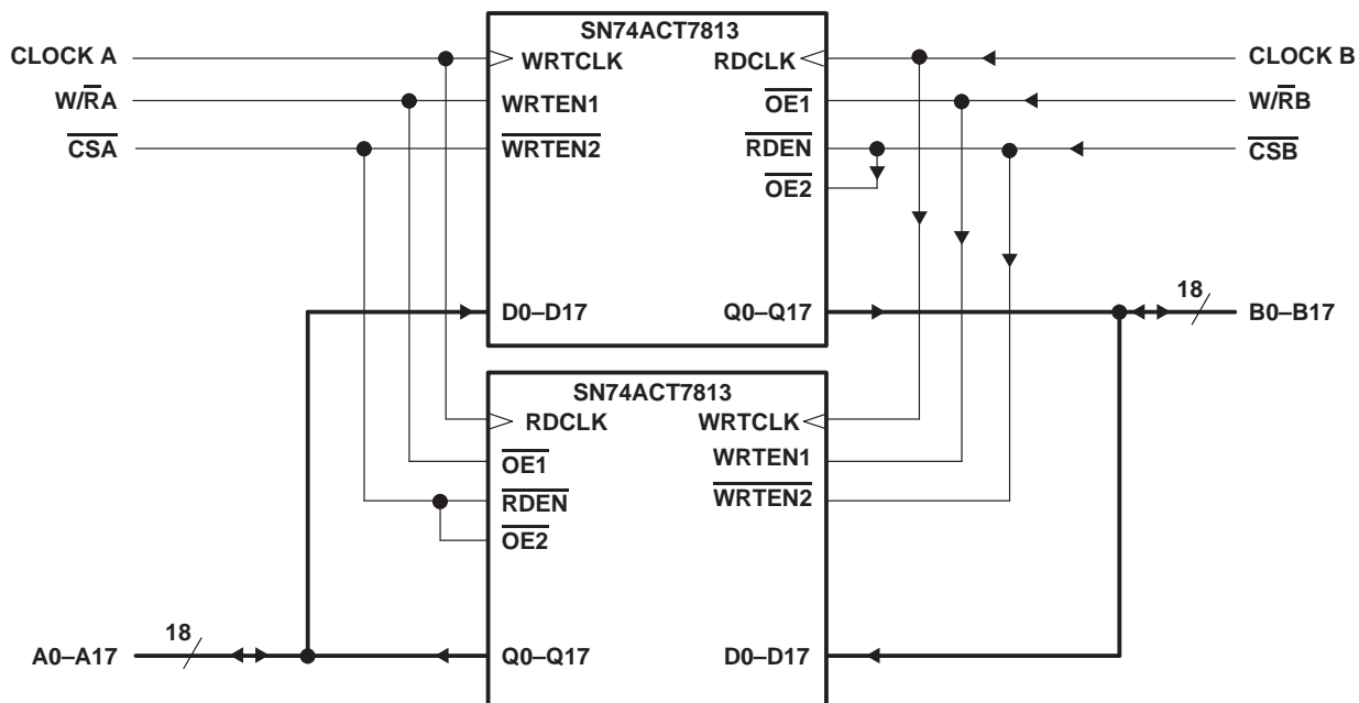
Figure 8. Bidirectional Configuration
