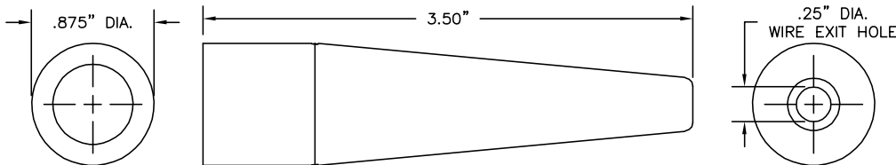
Insulation Boot P/N 9352-color
