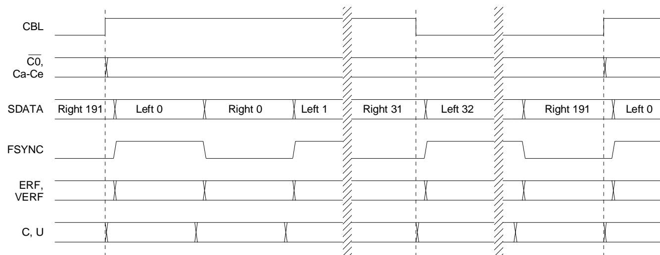
Figure 19. CBL Timing
