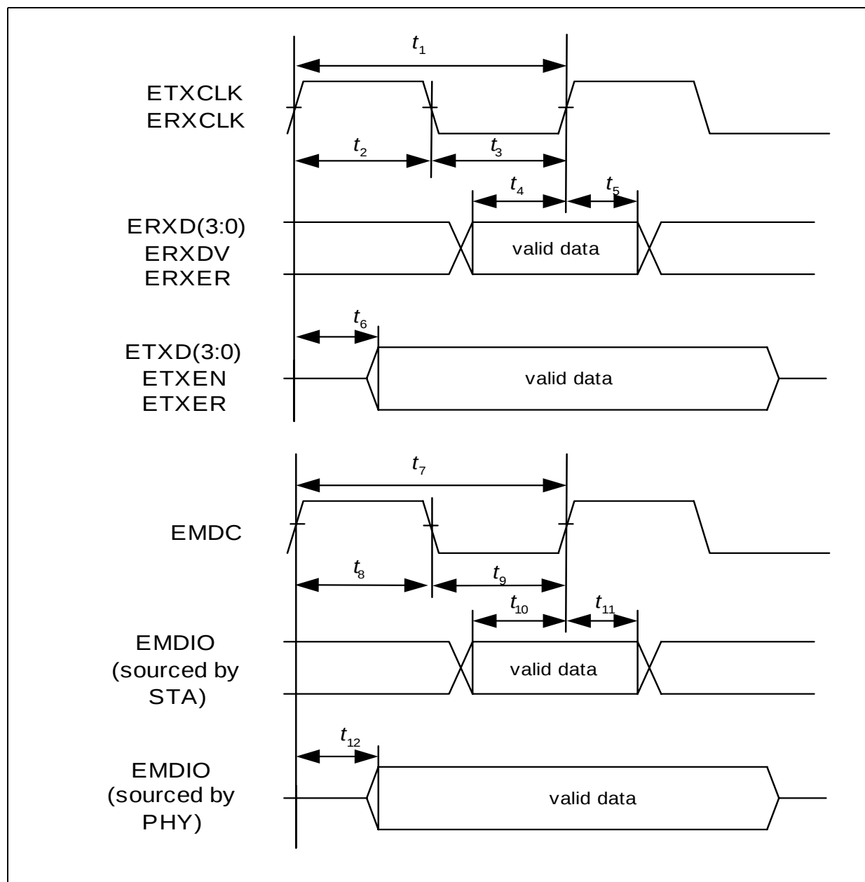
Figure 4-15 Ethernet Timing
