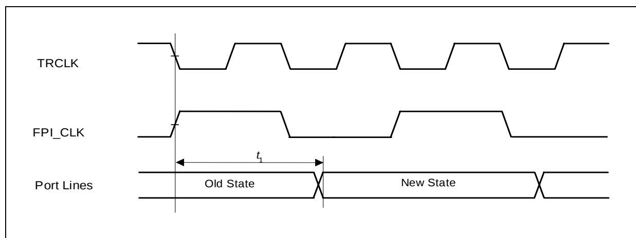
Figure 4-6 Port Timing
