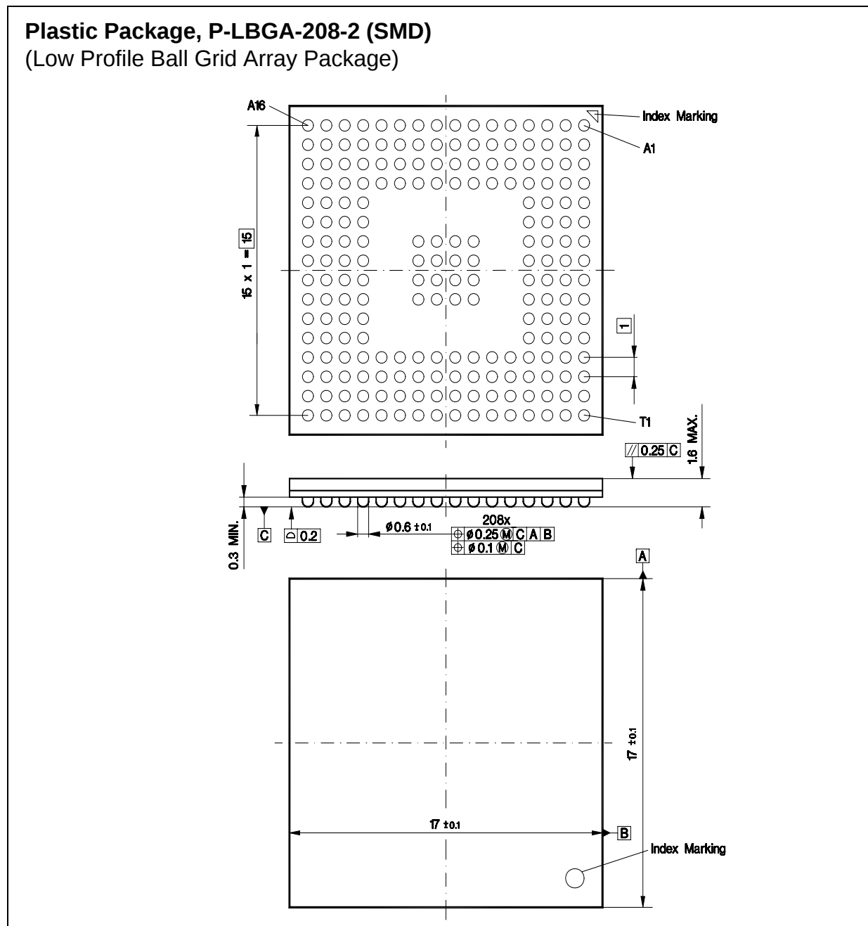
Figure 4-19 P-LBGA-208-2 Package
