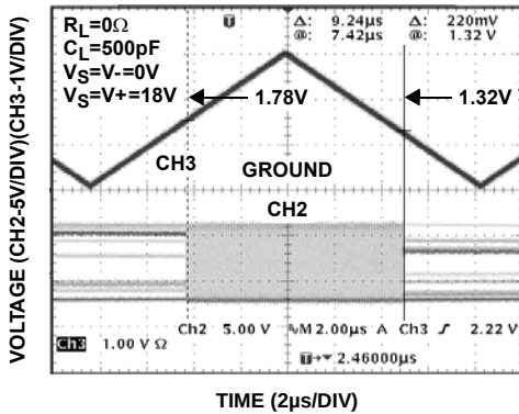
FIGURE 11. ENABLE/DISABLE THRESHOLD
