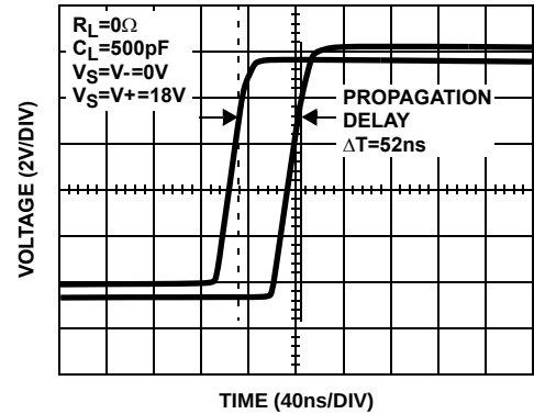
FIGURE 12. PROPAGATION DELAY
