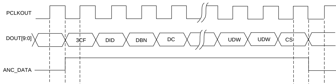
Fig. 10b \text{ANC\_DATA} Timing for Composite Signals
