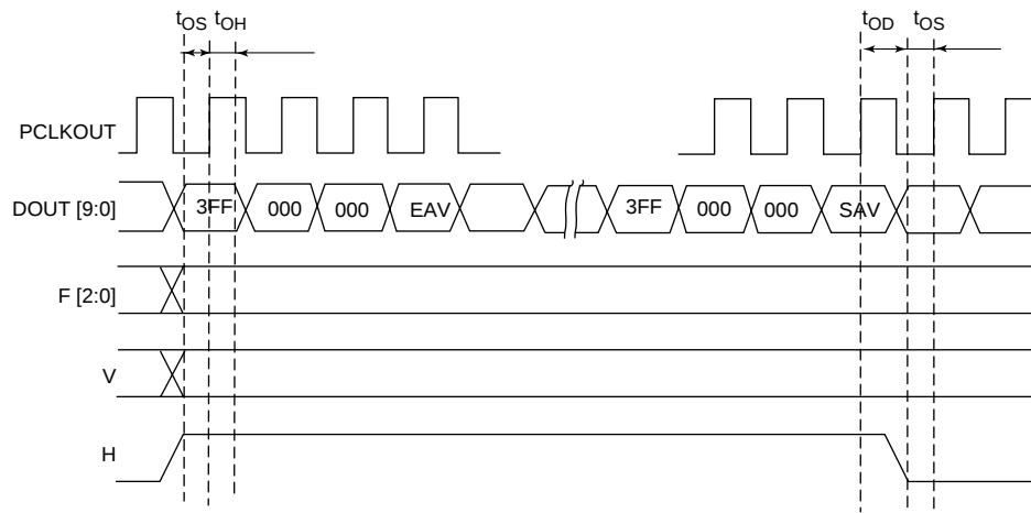
Fig. 8a FVH Timing for Component Video
