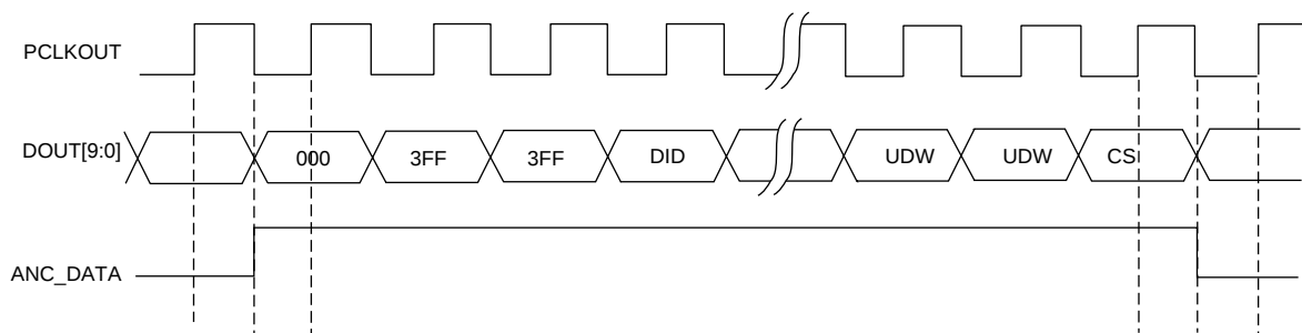
Fig. 10a \text{ANC\_DATA} Timing for Component Signals
