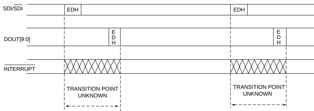
Fig. 11 \text{INTERRUPT} Timing
