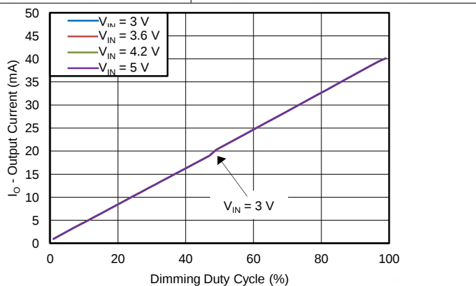
Figure 5. Dimming Linearity
