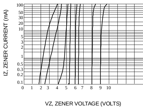
Fig. 7-VZ = 6.8 THRU 10 VOLTS
