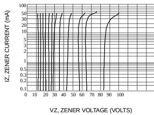
Fig. 8-VZ = 12 THRU 82 VOLTS
