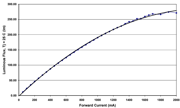
Warm White with Built-in 60° Optic (NT-45D1-0446)
