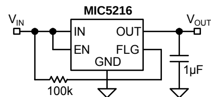
Figure 5. Low-Noise Fixed Voltage Regulator
