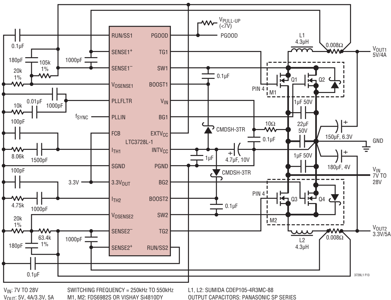
Figure 13. LTC3728L-1 5V/4A, 3.3V/5A Regulator with External Frequency Synchronization
