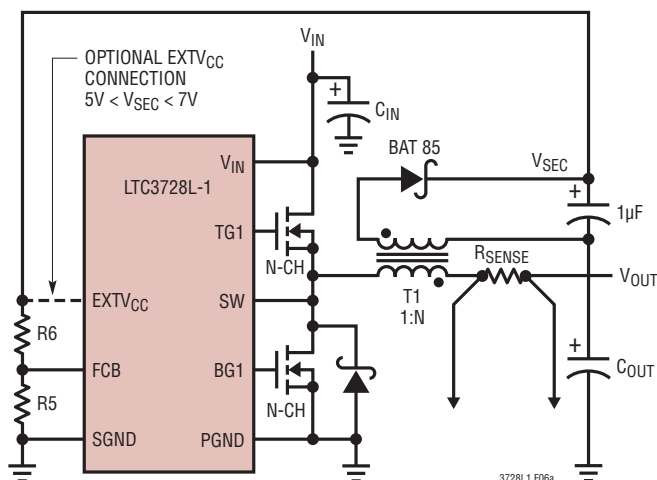
Figure 6a. Secondary Output Loop & EXT V CC Connection
