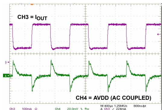
FIGURE 7. BOOST TRANSIENT RESPONSE @ 1.3MHz
