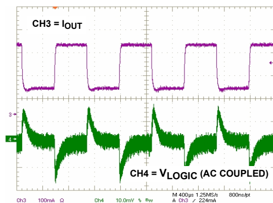
FIGURE 12. BUCK TRANSIENT RESPONSE @ 650kHz
