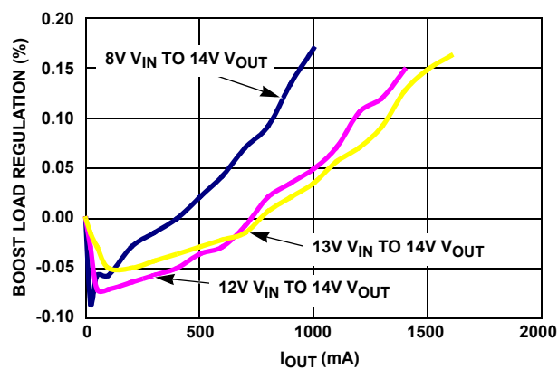
FIGURE 4. BOOST LOAD REGULATION @ 1.3MHz
