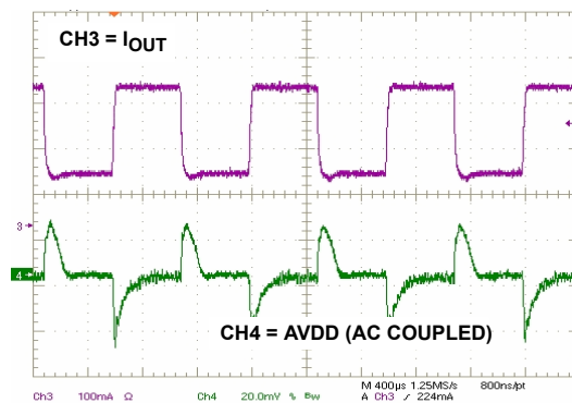
FIGURE 6. BOOST TRANSIENT RESPONSE @ 650kHz
