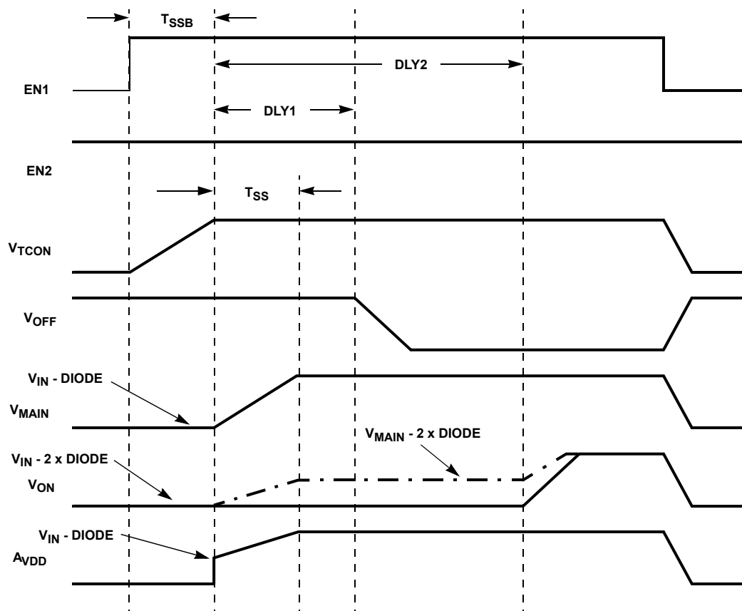
FIGURE 23. TIMING DIAGRAM 2
