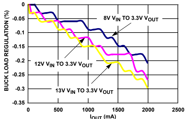
FIGURE 10. BUCK LOAD REGULATION @ 650kHz
