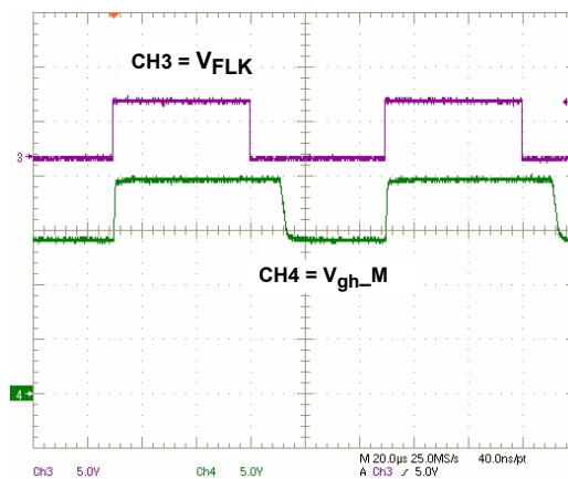
FIGURE 16. GPM WAVEFORM
