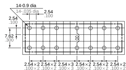
PC board pattern (Copper-side view) Single side stable, 1 coil latching
