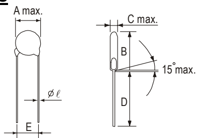
Dimension Table
