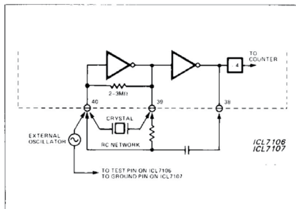
Figure 7. Clock Circuits
