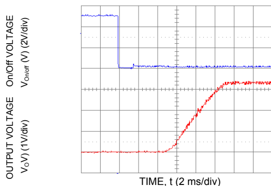
Figure 15. Typical Start-Up Using Remote On/Off with Low-ESR external capacitors (7x150µF Polymer) ( V_{in} = 5.0\text{Vdc} , V_o = 3.3\text{Vdc} , I_o = 6\text{A} , C_o = 1050\text{ }\mu\text{F} ).
