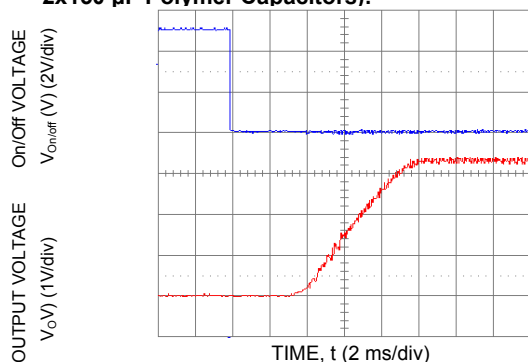
Figure 14. Typical Start-Up Using Remote On/Off ( V_{in} = 5.0\text{Vdc} , V_o = 3.3\text{Vdc} , I_o = 6\text{A} ).
