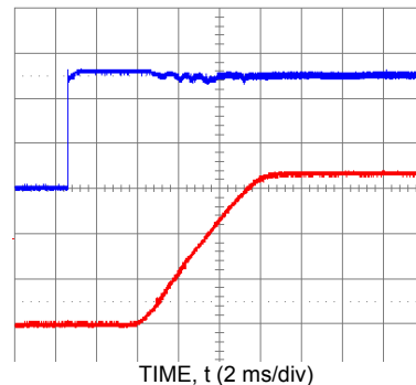
Figure 16. Typical Start-Up with application of V_{in} ( V_{in} = 5.0\text{Vdc} , V_o = 3.3\text{Vdc} , I_o = 6\text{A} ).
