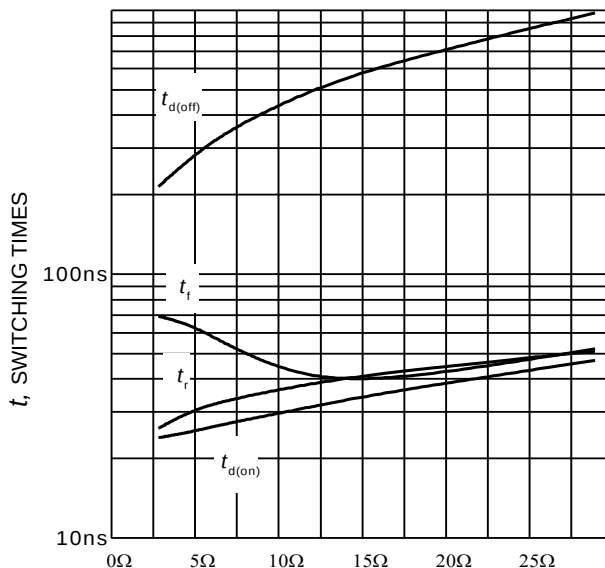
Figure 10. Typical switching times as a function of gate resistor (inductive load, T_J = 175^\circ\text{C} , V_{CE} = 400\text{V} , V_{GE} = 0/15\text{V} , I_C = 50\text{A} , Dynamic test circuit in Figure E)
