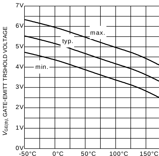
Figure 12. Gate-emitter threshold voltage as a function of junction temperature ( I_C = 0.8\text{mA} )
