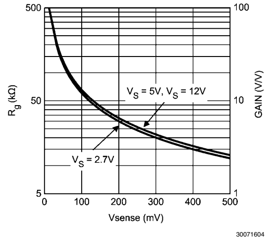
FIGURE 2. Allowed Gains for Range 1
