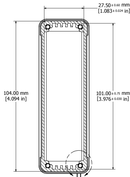
SECTION T-T
