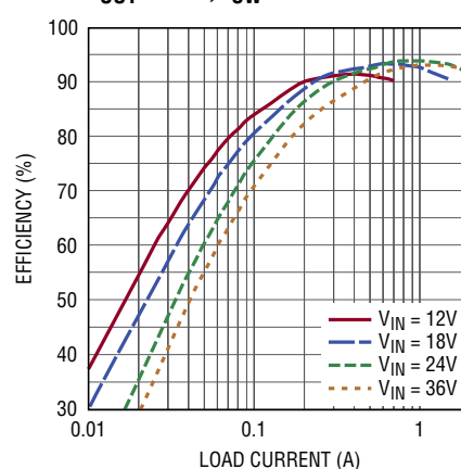
PWM Mode Efficiency, V_{OUT} = 24V , f_{SW} = 1\text{MHz}
