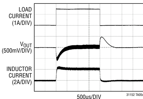
0A to 1.5A Load Step, V IN = 20V
