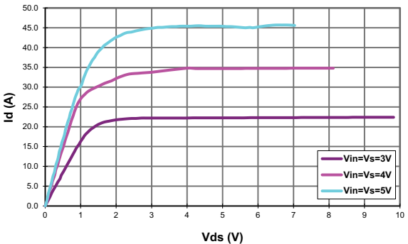
Figure 10. Output characteristics ( T_{\text{case}} = 25^{\circ}\text{C} )
