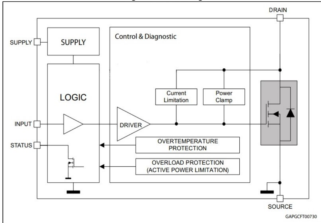
Figure 1. Block diagram
