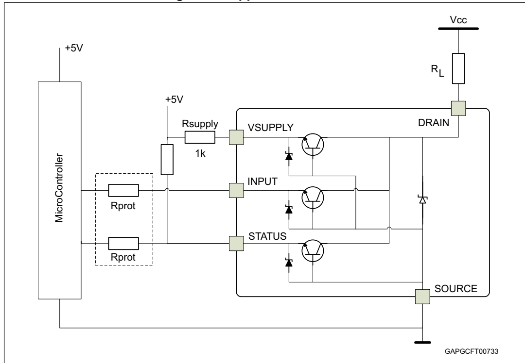
Figure 14. Application schematic
