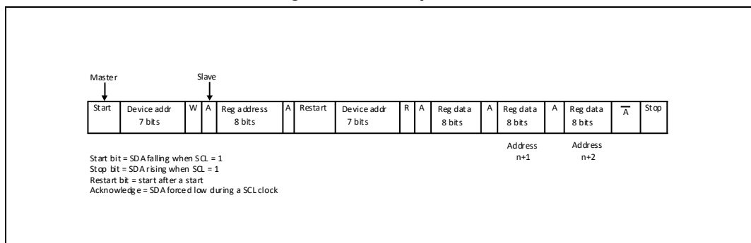
Figure 4. Read operation
