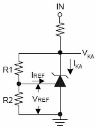
Figure 2. V_{ka} > V_{ref}
