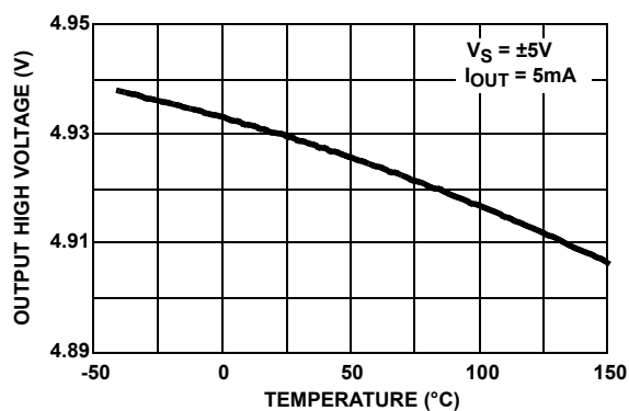
FIGURE 6. OUTPUT HIGH VOLTAGE vs TEMPERATURE
