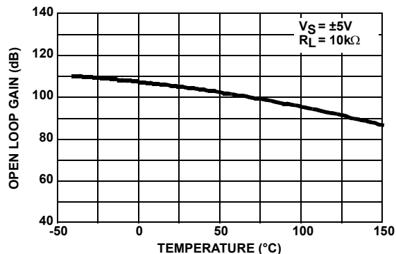
FIGURE 8. OPEN-LOOP GAIN vs TEMPERATURE
