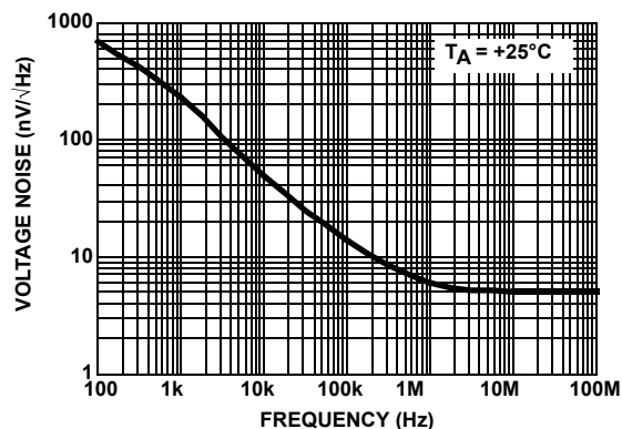
FIGURE 20. INPUT VOLTAGE NOISE SPECTRAL DENSITY vs FREQUENCY
