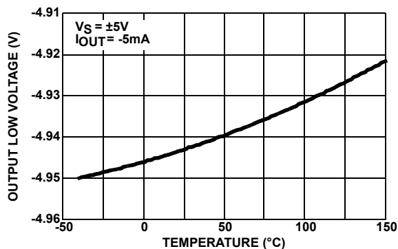
FIGURE 7. OUTPUT LOW VOLTAGE vs TEMPERATURE
