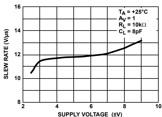
FIGURE 12. SLEW RATE vs SUPPLY VOLTAGE
