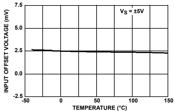
FIGURE 4. INPUT OFFSET VOLTAGE vs TEMPERATURE
