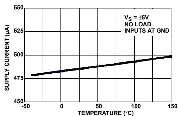
FIGURE 10. SUPPLY CURRENT PER AMPLIFIER vs TEMPERATURE
