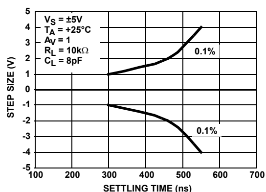
FIGURE 24. STEP SIZE vs SETTLING TIME
