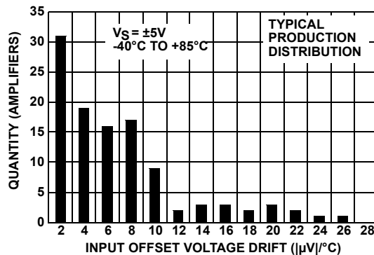
FIGURE 2. INPUT OFFSET VOLTAGE DRIFT (TSSOP, SOIC)
