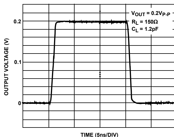
FIGURE 15. SMALL SIGNAL TRANSIENT RESPONSE; R_L = 150\Omega
