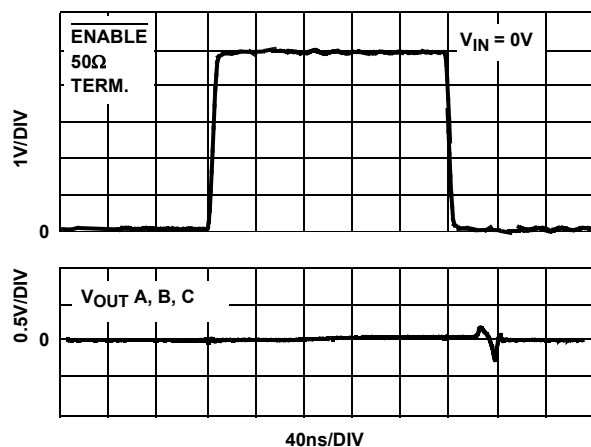
FIGURE 22. \overline{\text{ENABLE}} SWITCHING GLITCH V_{IN} = 0V
