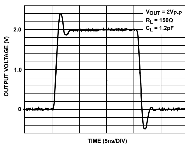
FIGURE 17. LARGE SIGNAL TRANSIENT RESPONSE; R_L = 150\Omega
