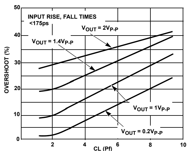
FIGURE 19. PULSE OVERSHOOT vs V_{OUT} , C_L ; R_L = 150\Omega
